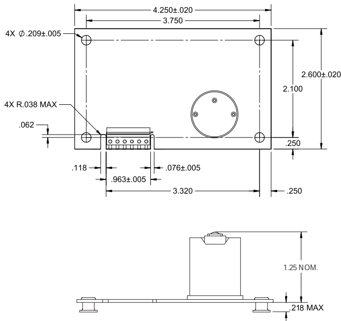
Figure 5. Board Dimensions
