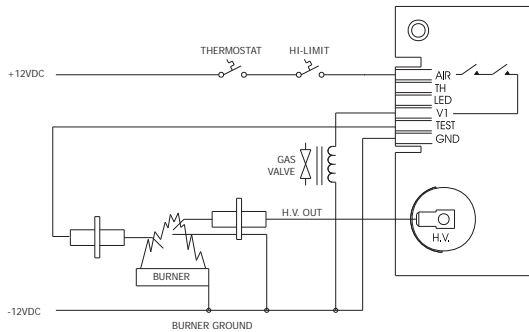
Figure 4. Remote Sense without Blower Relay
