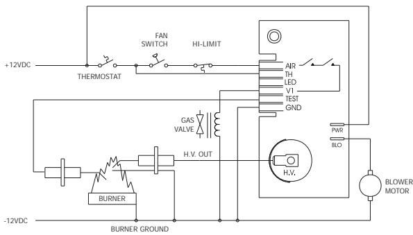
Figure 3. Remote Sense with Blower Relay
