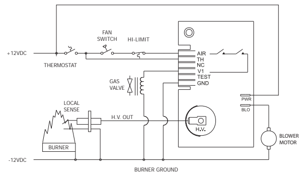
Figure 1. Local Sense with Blower Relay
