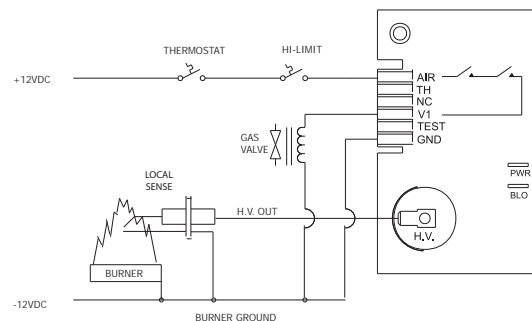
Figure 2. Local Sense without Blower Relay
