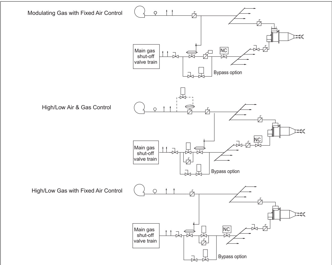
Figure 3.5 Bypass Start Gas Circuit Schematics
