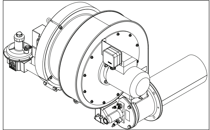
Figure 1.1. ThermAir Burner
