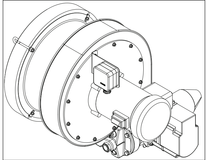
Figure 1.1 RatioAir Burner
