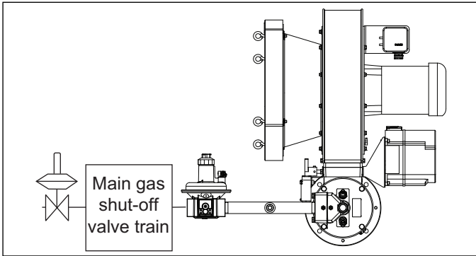
Figure 3.6. Low Fire Start
