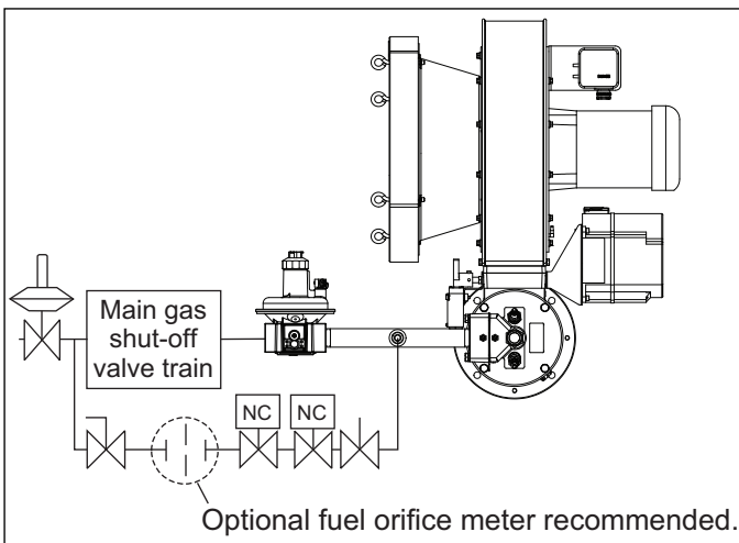
Figure 3.7. Pilot Start (Optional)
