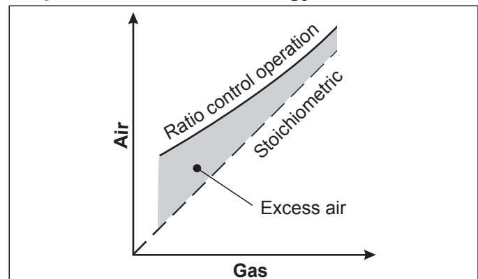
Figure 3.3. Air : Gas Flow
