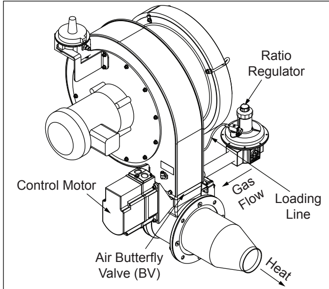
Figure 3.4. Basic Burner Components
