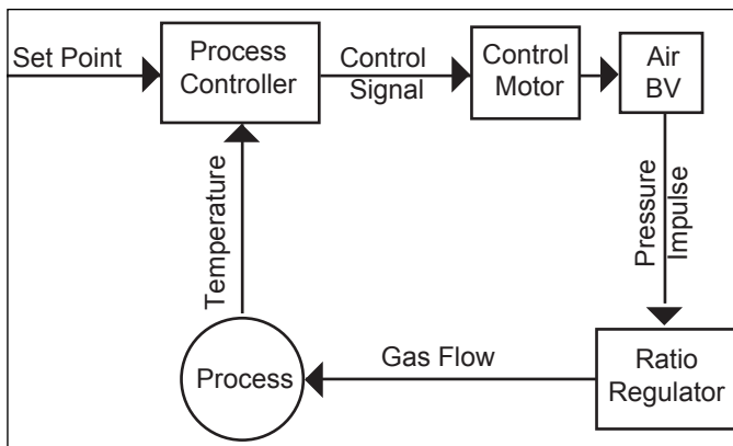
Figure 3.5. Basic Control Loop
