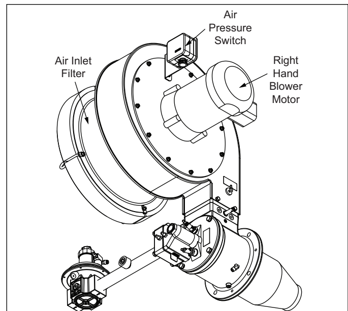
Figure 3.2. Burner Configuration & Motor Orientation Choice
